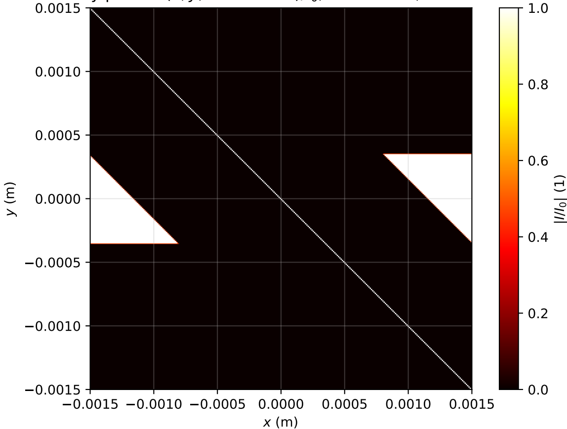
Intensity profile I(x, y, z = 0.000\text{m})/I_0 , \text{Pin}=2.0\text{Pcr} , artificial time
